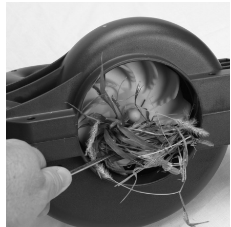
Figure 4-13: Removing debris from impellers
